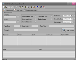
Search Loan
