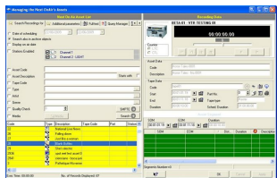
Main Window
